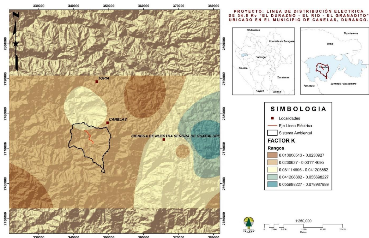
Figura IV. 26 Factor K
