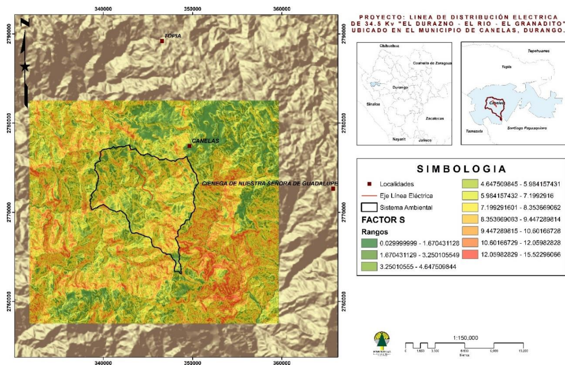
Figura IV. 34 Factor S
