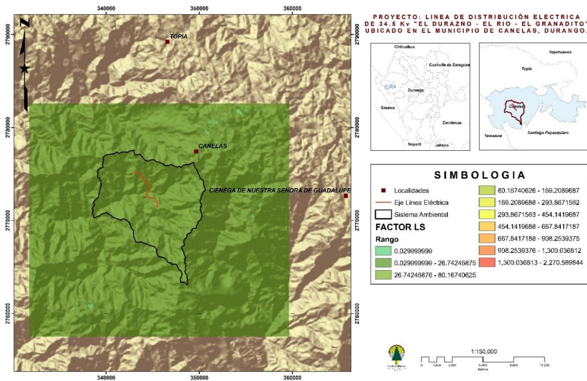
Figura IV. 35 Factor LS
