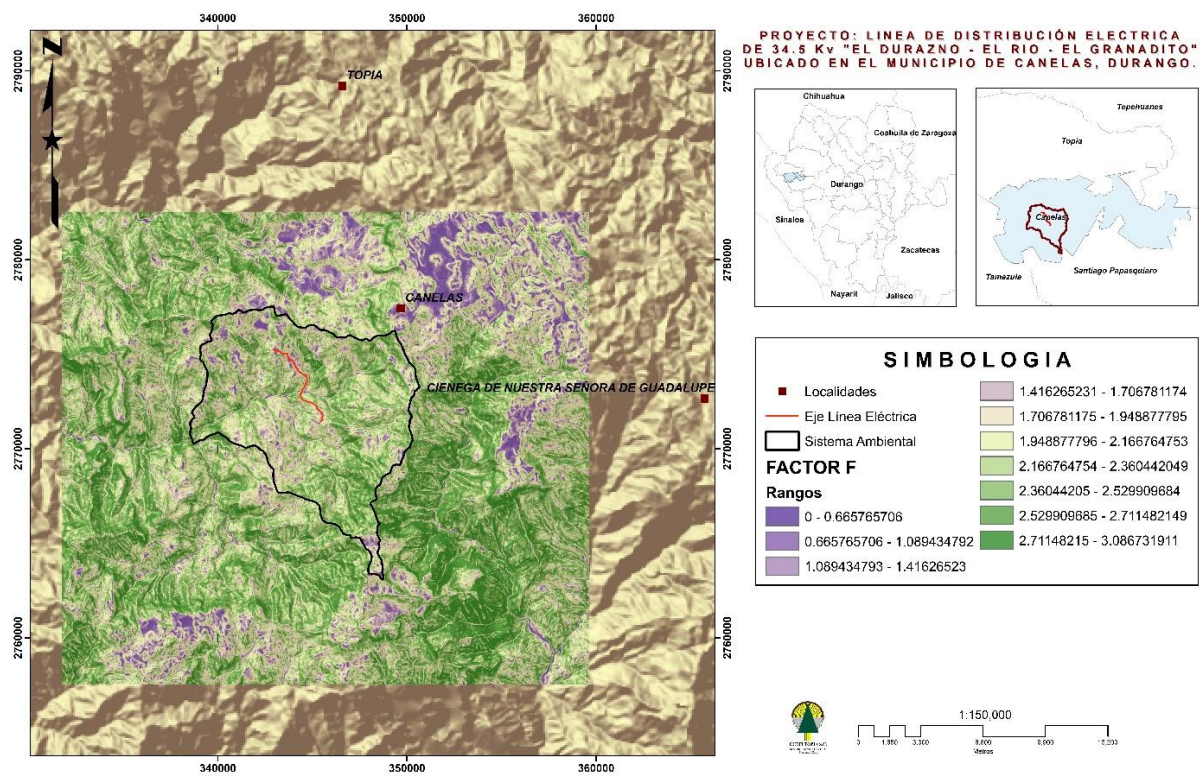
Figura IV. 29 Factor F
