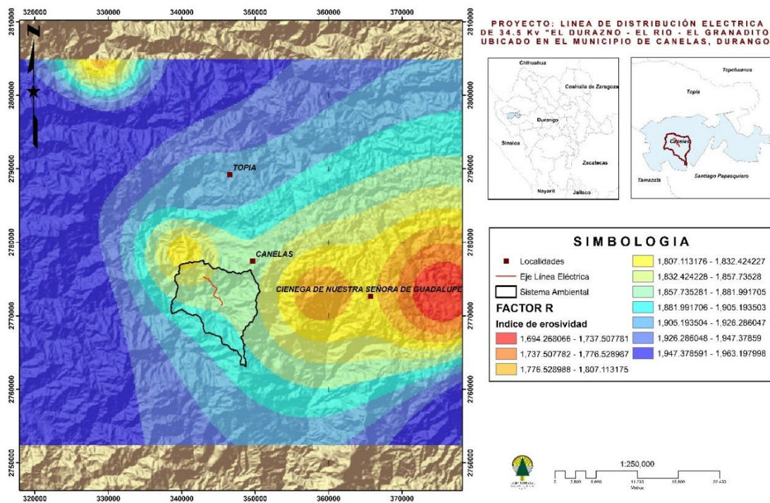
Figura IV. 25 Factor R
