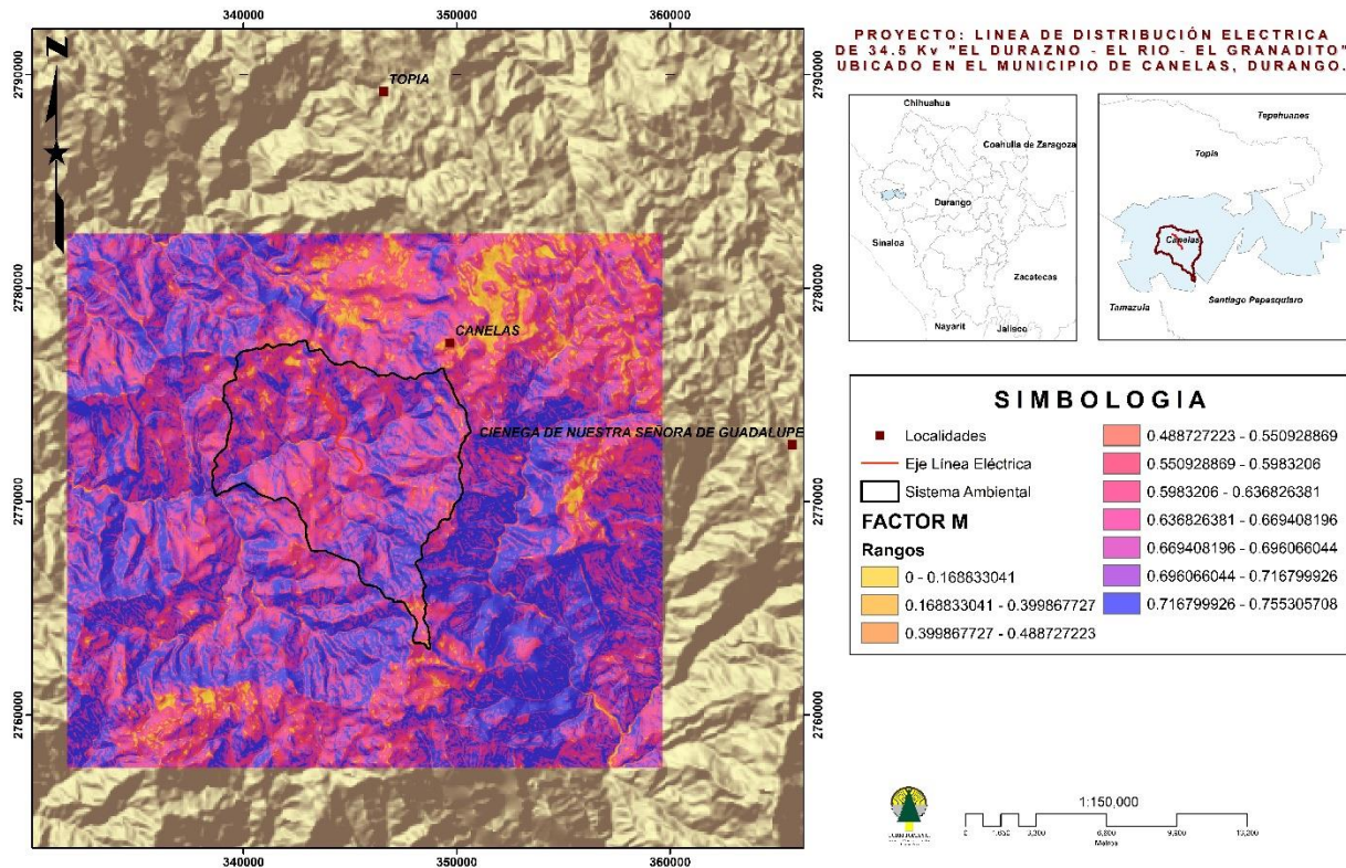
Figura IV. 30 Factor M
