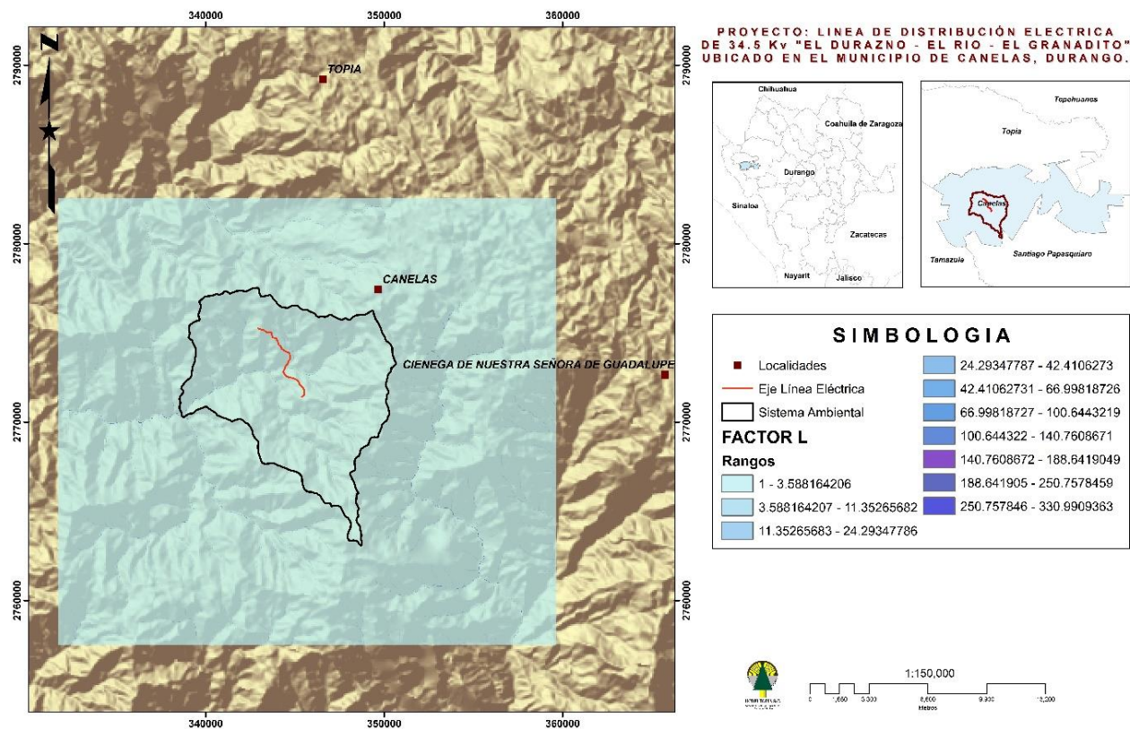
Figura IV. 33 Factor L
