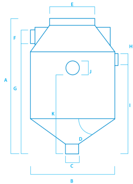
PLANO BIODIGESTOR RP-7000
